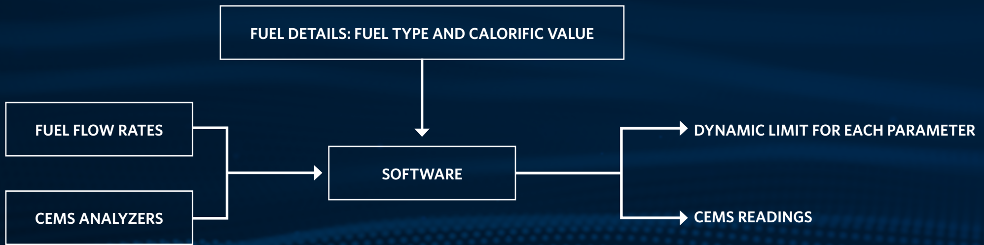
Figure A: Emission Model Conceptual Diagram, *CEMS Continuous Emission Monitoring System
