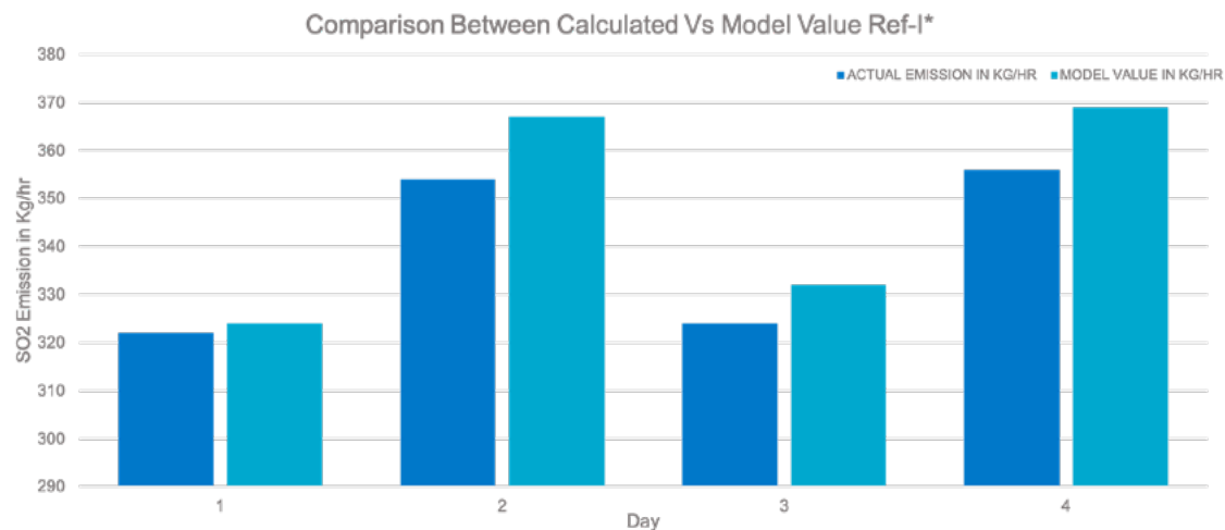
Figure E: SO 2 Emission from Ref-1 on 4 Various Sample Days
