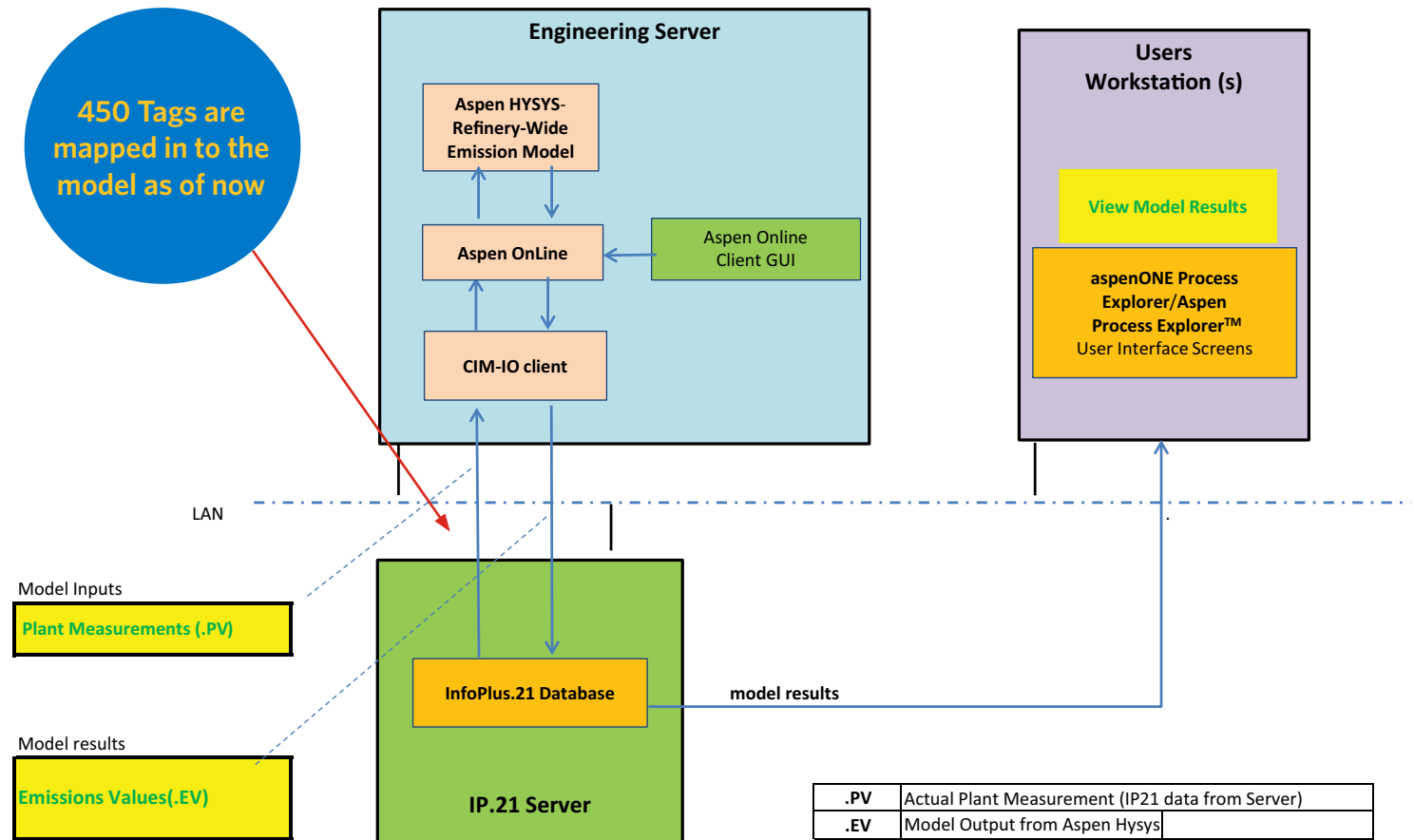
Figure D: Digital Twin System Architecture of Emission Model
