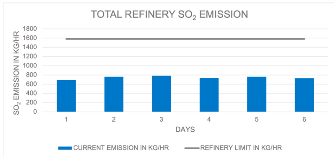
Figure F: SO 2 Total Refinery Emissions on Various Sample Days
